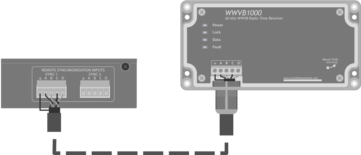
Figure 2.1 - WWVB1000 master clock connection
